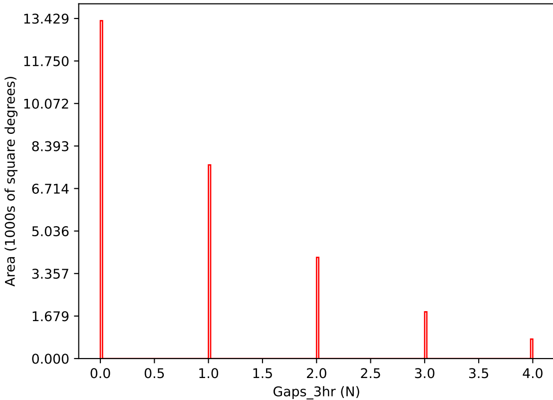
internal_u_expt30_nscale1.1v3.4_10yrs i band: Gaps_3hr
