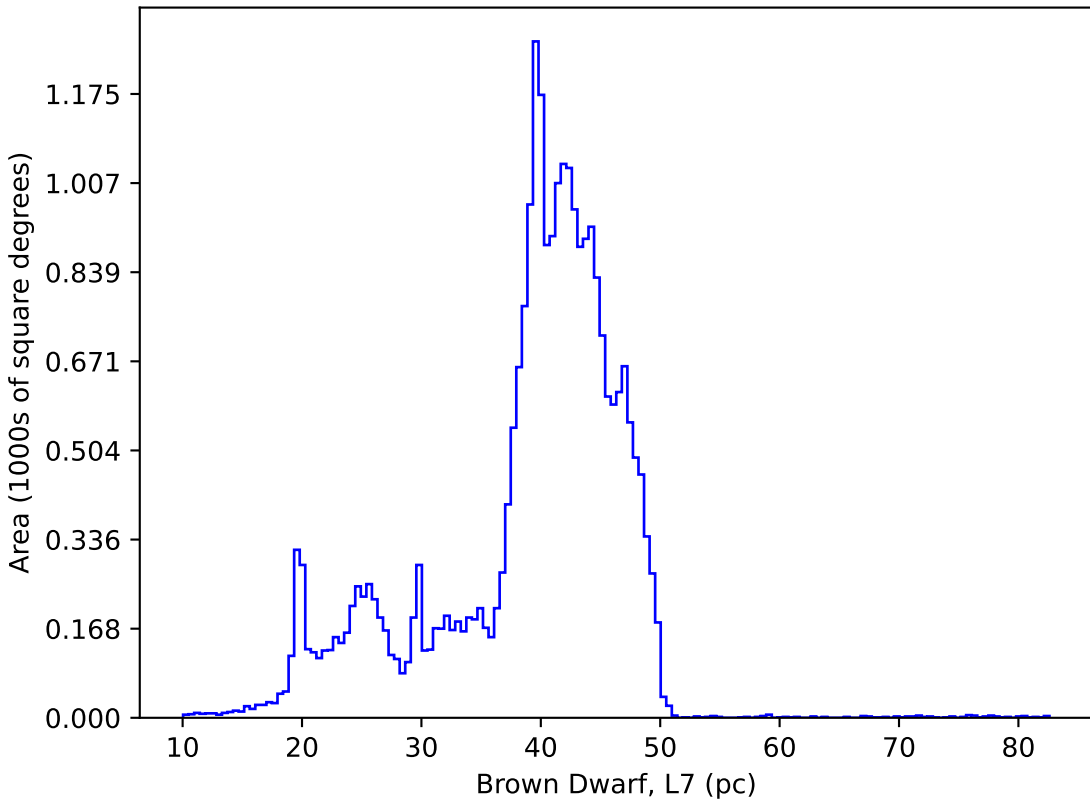
internal_u_expt30_nscale1.1v3.4_10yrs : Brown Dwarf, L7
