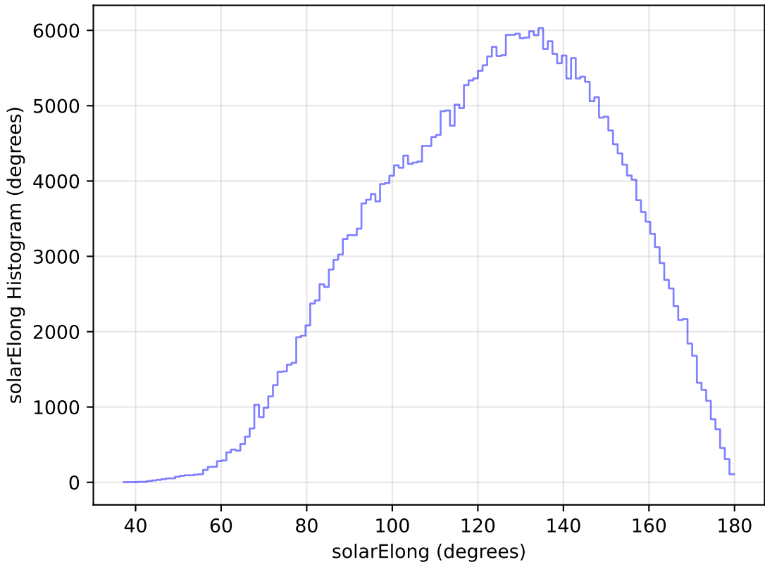
internal_u_expt30_nscale1.1v3.4_10yrs WFD y band: solarElong Histogram
