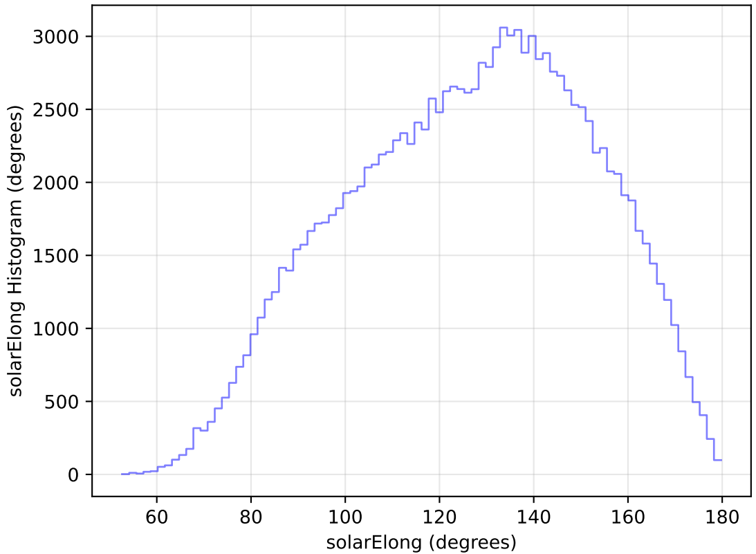
internal_u_expt30_nscale1.1v3.4_10yrs WFD u band: solarElong Histogram
