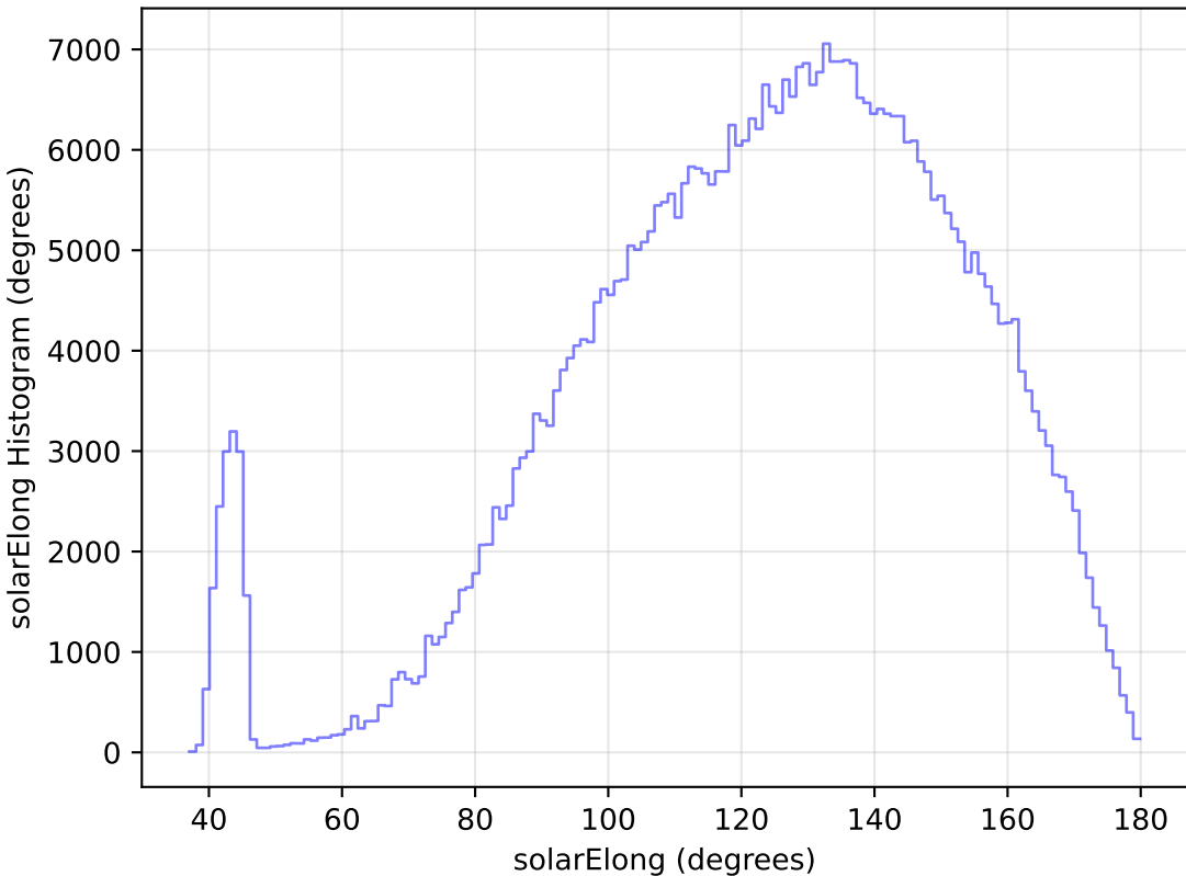
internal_u_expt30_nscale1.1v3.4_10yrs WFD r band: solarElong Histogram
