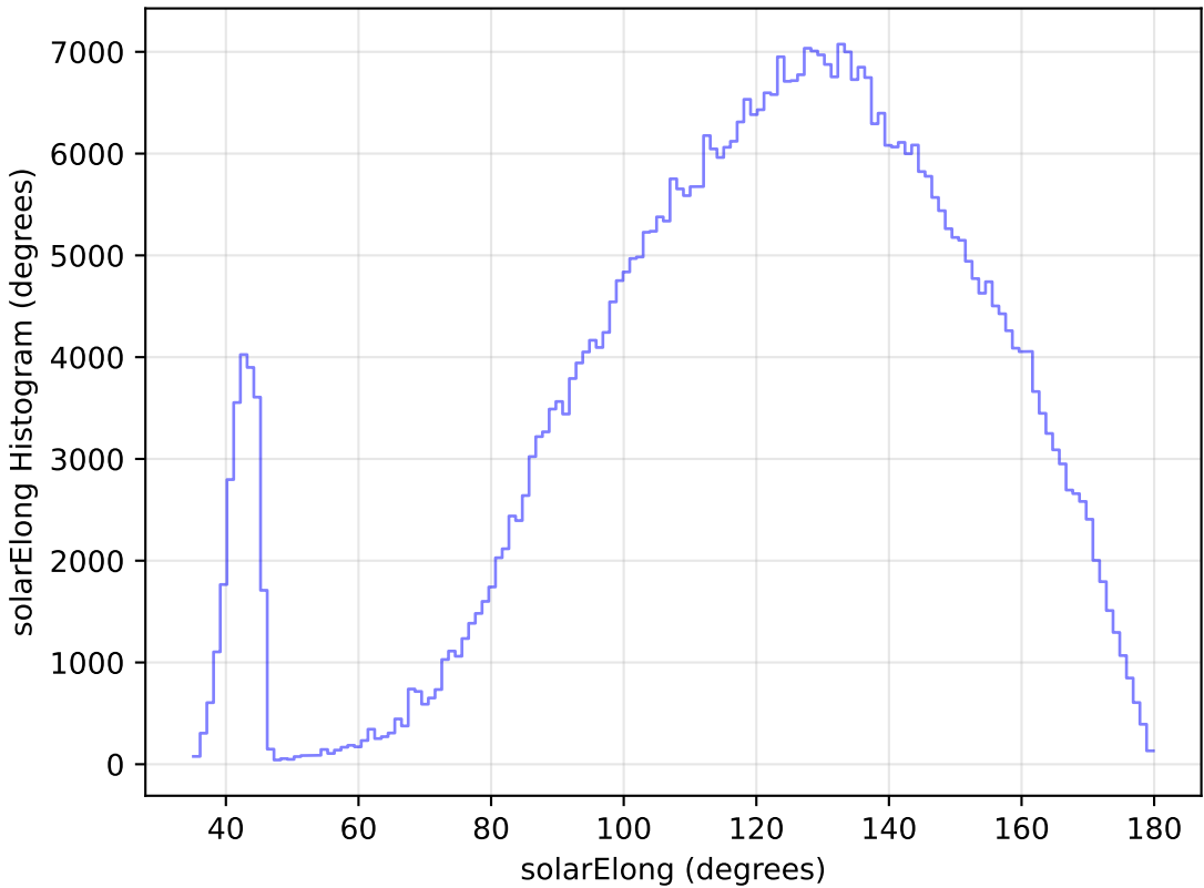
internal_u_expt30_nscale1.1v3.4_10yrs WFD i band: solarElong Histogram
