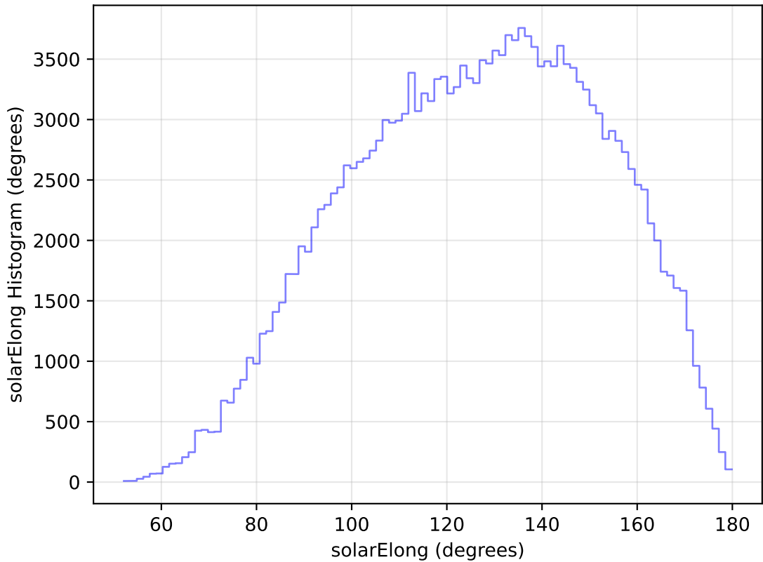
internal_u_expt30_nscale1.1v3.4_10yrs WFD g band: solarElong Histogram
