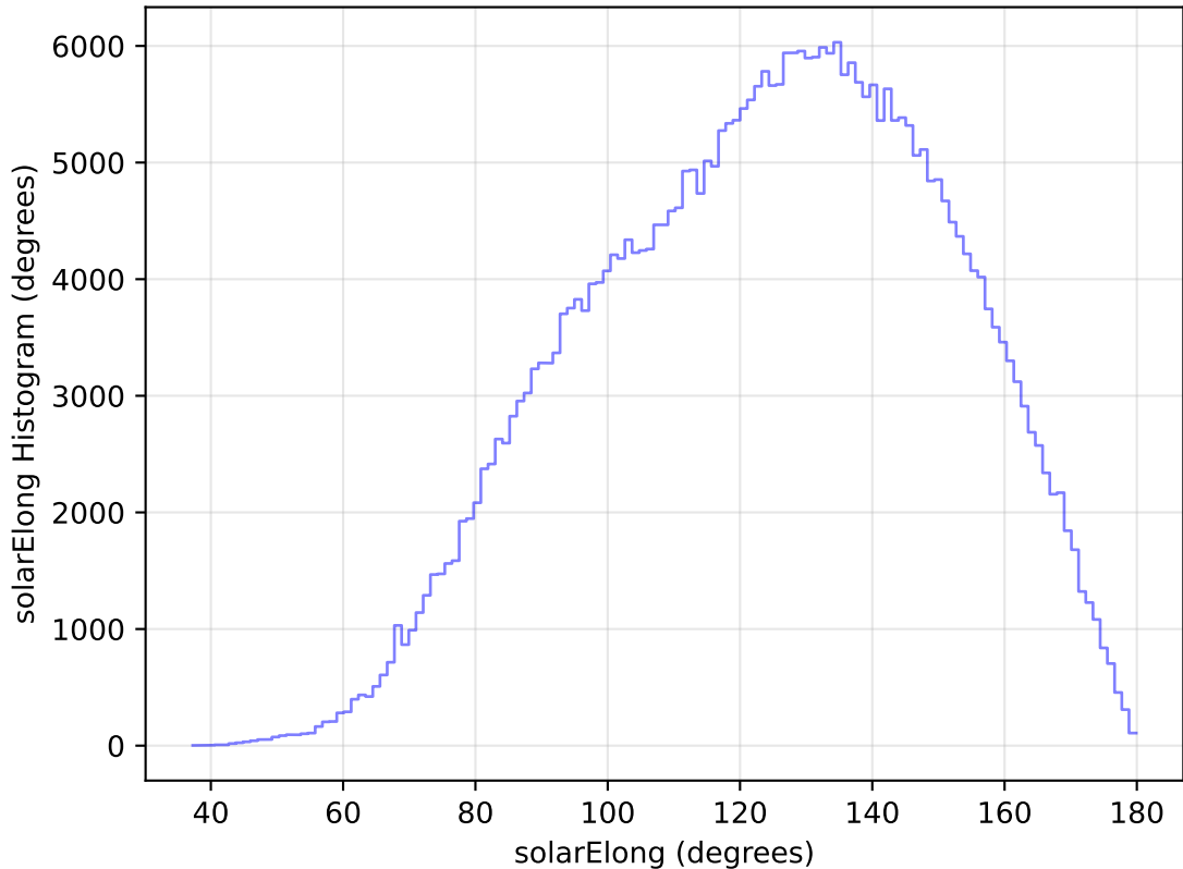
internal_u_expt30_nscale1.1v3.4_10yrs All sky y band: solarElong Histogram
