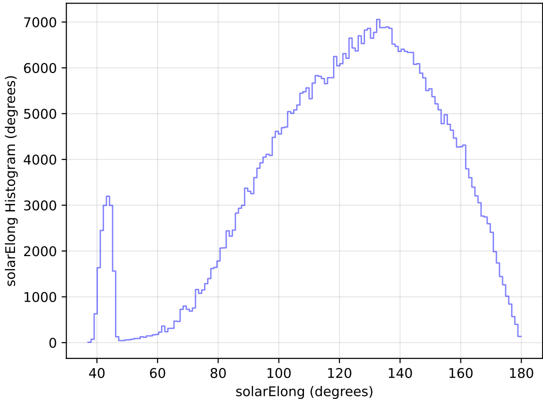
internal_u_expt30_nscale1.1v3.4_10yrs All sky r band: solarElong Histogram
