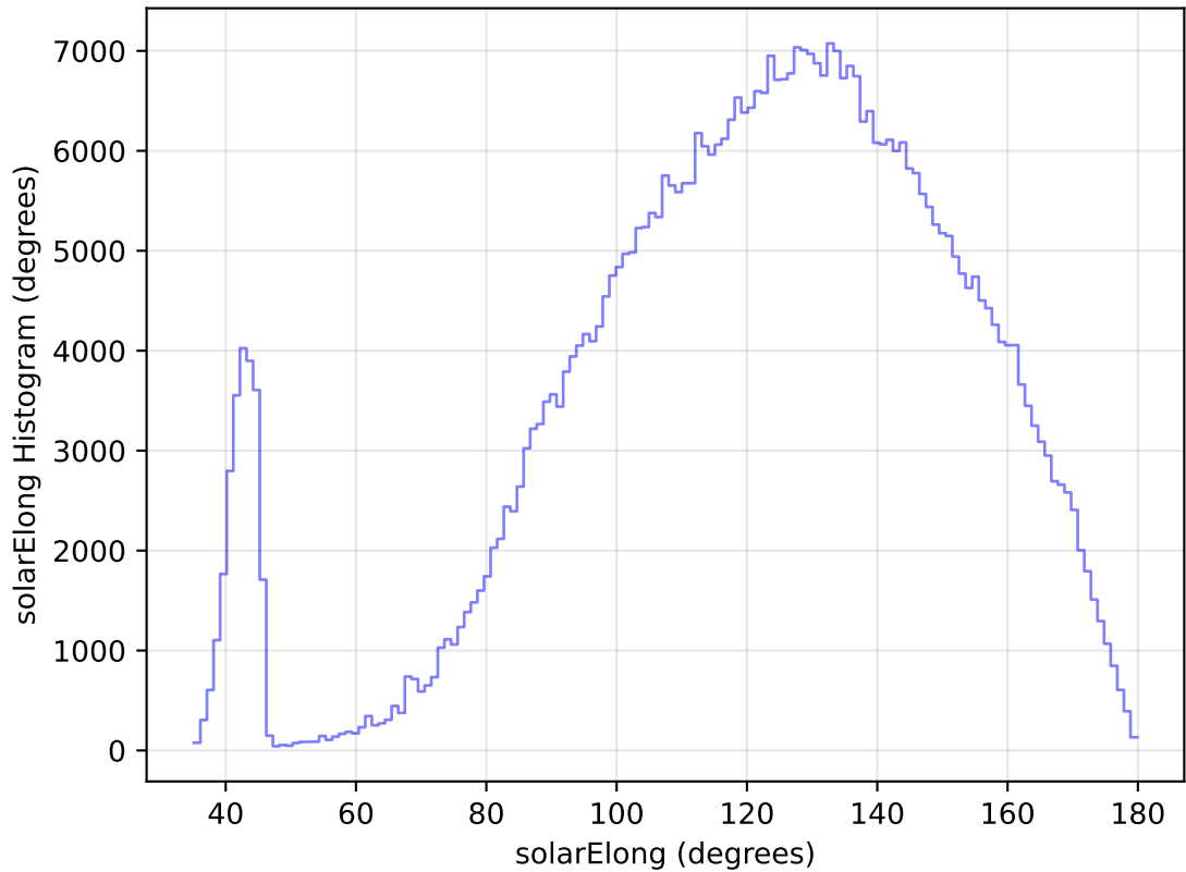
internal_u_expt30_nscale1.1v3.4_10yrs All sky i band: solarElong Histogram
