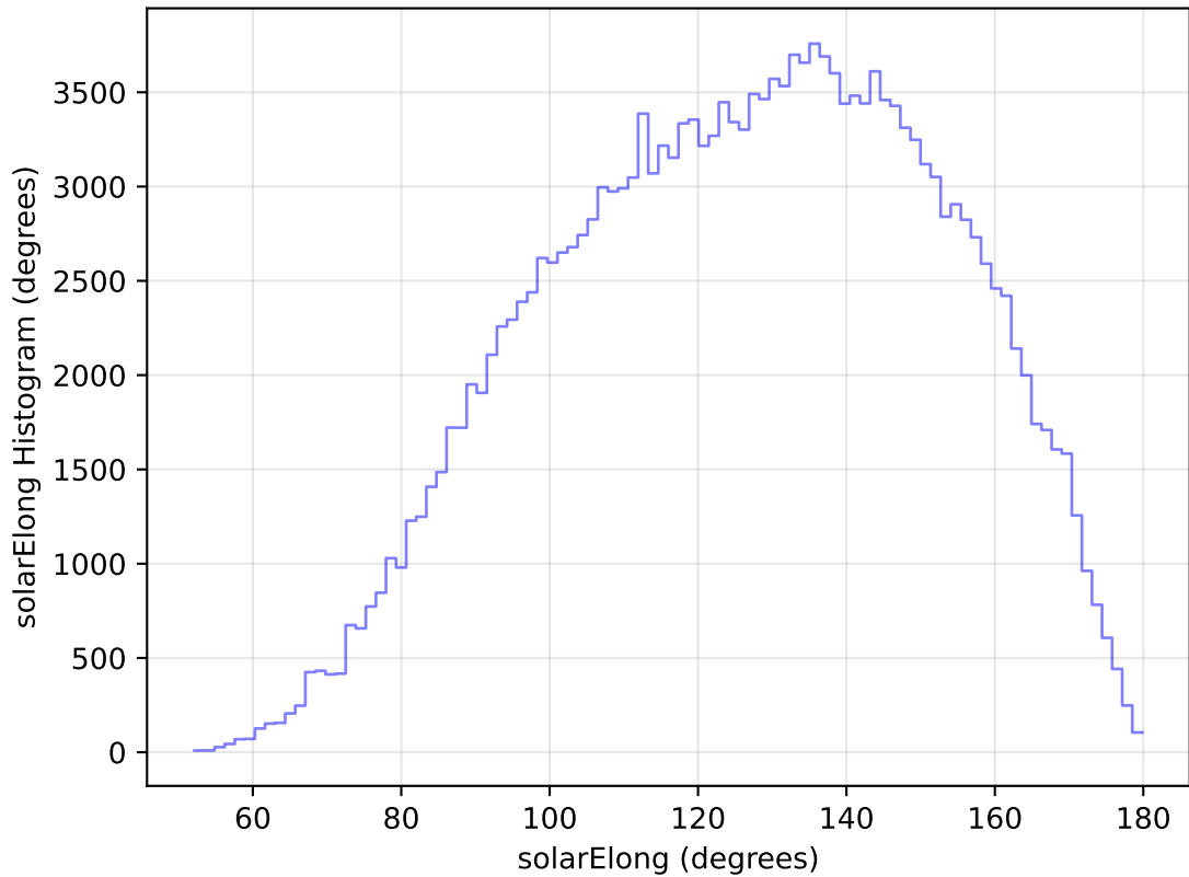
internal_u_expt30_nscale1.1v3.4_10yrs All sky g band: solarElong Histogram
