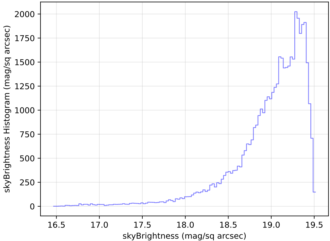
internal_u_expt30_nscale1.1v3.4_10yrs Yr 1 z band: skyBrightness Histogram
