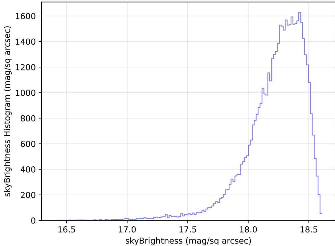
internal_u_expt30_nscale1.1v3.4_10yrs Yr 1 y band: skyBrightness Histogram
