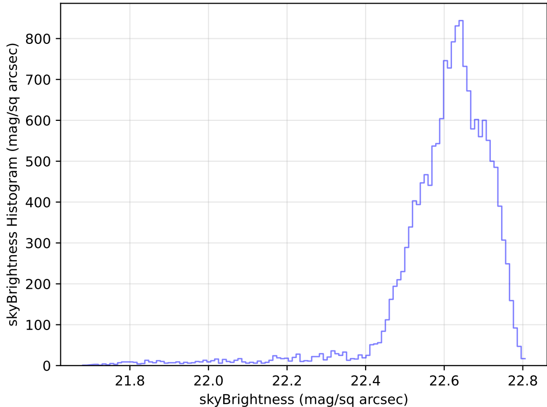
internal_u_expt30_nscale1.1v3.4_10yrs Yr 1 u band: skyBrightness Histogram
