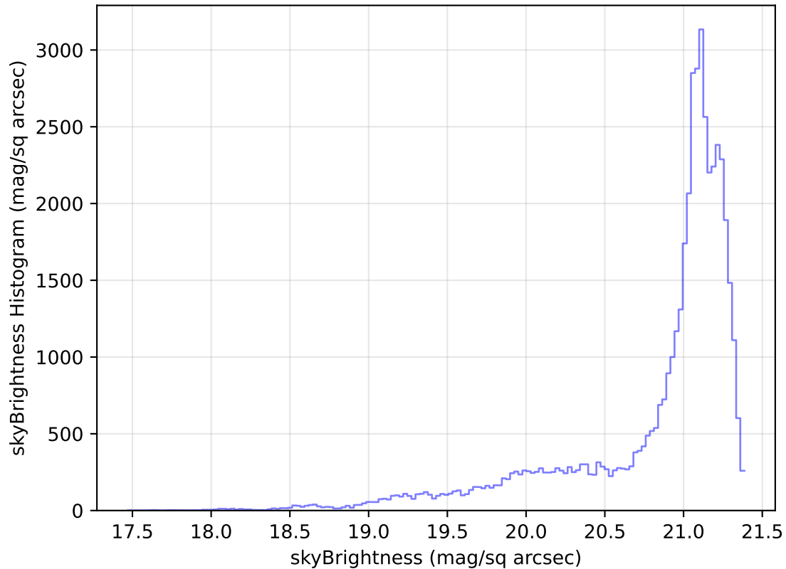
internal_u_expt30_nscale1.1v3.4_10yrs Yr 1 r band: skyBrightness Histogram
