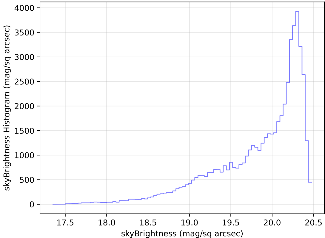
internal_u_expt30_nscale1.1v3.4_10yrs Yr 1 i band: skyBrightness Histogram
