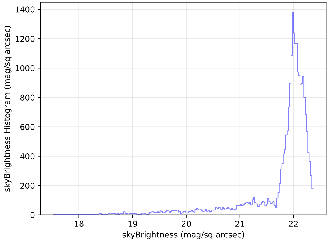
internal_u_expt30_nscale1.1v3.4_10yrs Yr 1 g band: skyBrightness Histogram
