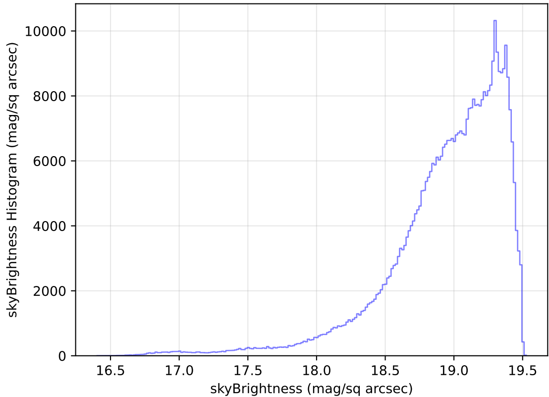
internal_u_expt30_nscale1.1v3.4_10yrs WFD z band: skyBrightness Histogram
