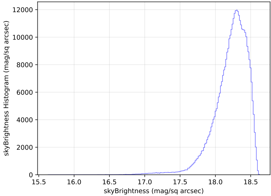
internal_u_expt30_nscale1.1v3.4_10yrs WFD y band: skyBrightness Histogram
