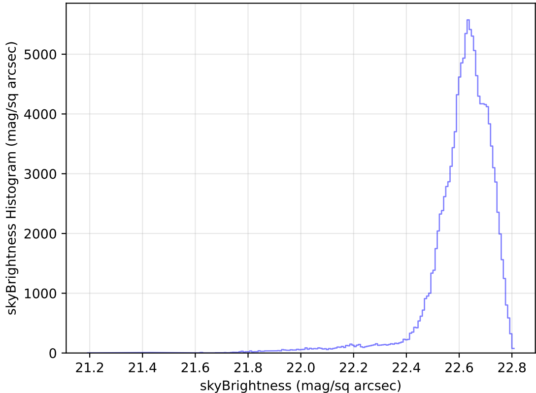
internal_u_expt30_nscale1.1v3.4_10yrs WFD u band: skyBrightness Histogram
