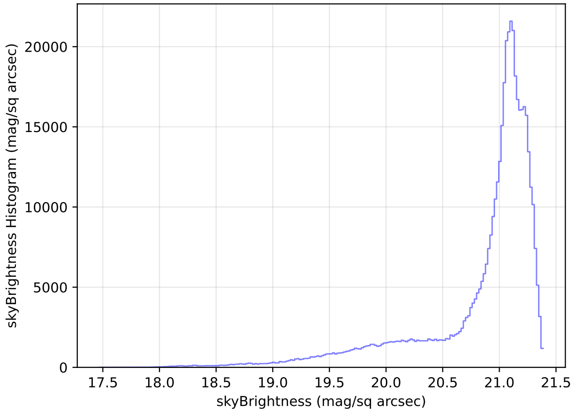
internal_u_expt30_nscale1.1v3.4_10yrs WFD r band: skyBrightness Histogram
