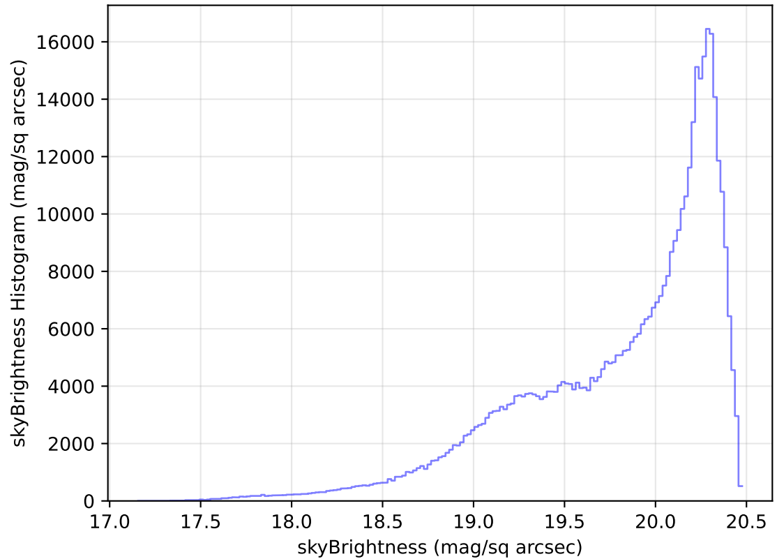
internal_u_expt30_nscale1.1v3.4_10yrs WFD i band: skyBrightness Histogram
