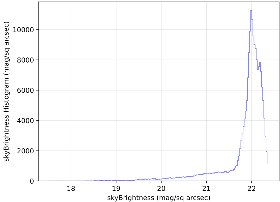
internal_u_expt30_nscale1.1v3.4_10yrs WFD g band: skyBrightness Histogram
