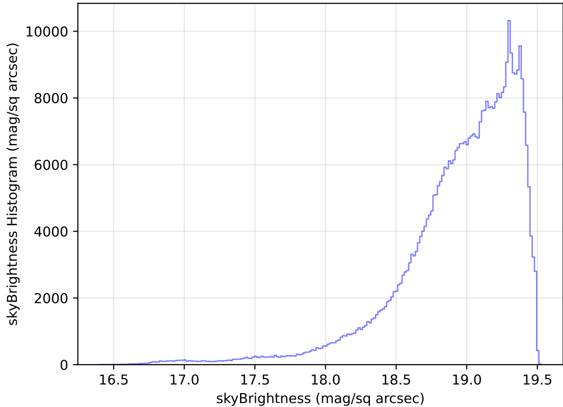
internal_u_expt30_nscale1.1v3.4_10yrs All sky z band: skyBrightness Histogram
