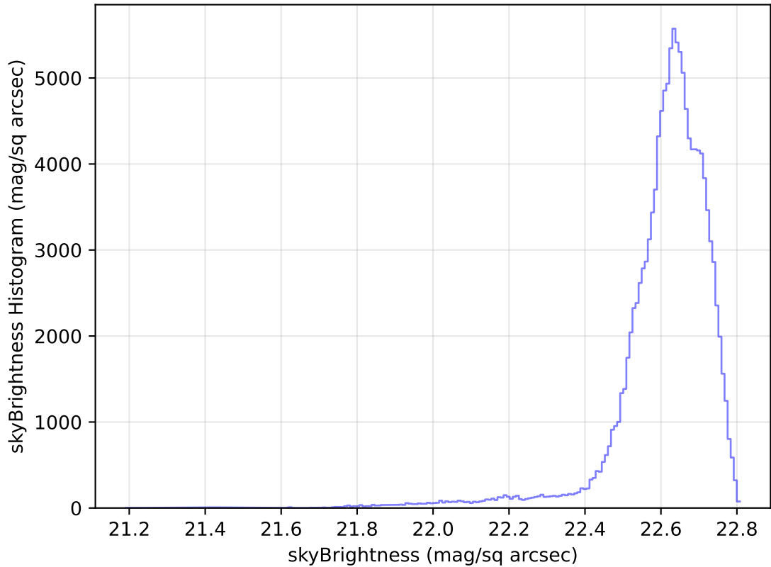
internal_u_expt30_nscale1.1v3.4_10yrs All sky u band: skyBrightness Histogram
