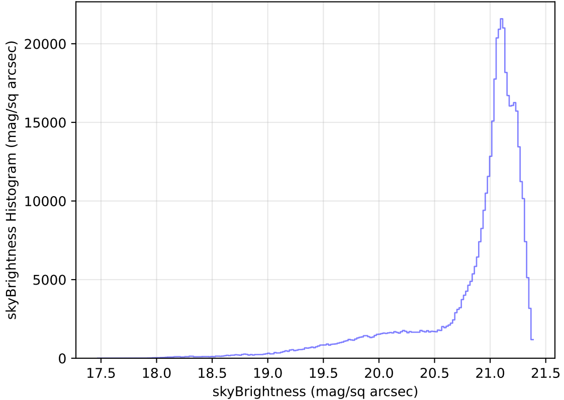
internal_u_expt30_nscale1.1v3.4_10yrs All sky r band: skyBrightness Histogram
