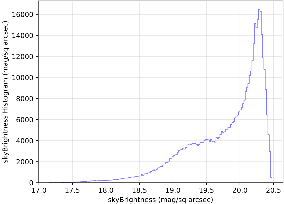
internal_u_expt30_nscale1.1v3.4_10yrs All sky i band: skyBrightness Histogram
