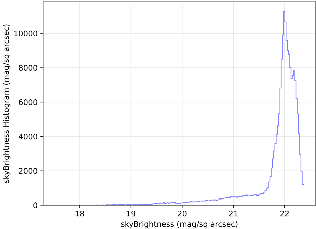
internal_u_expt30_nscale1.1v3.4_10yrs All sky g band: skyBrightness Histogram
