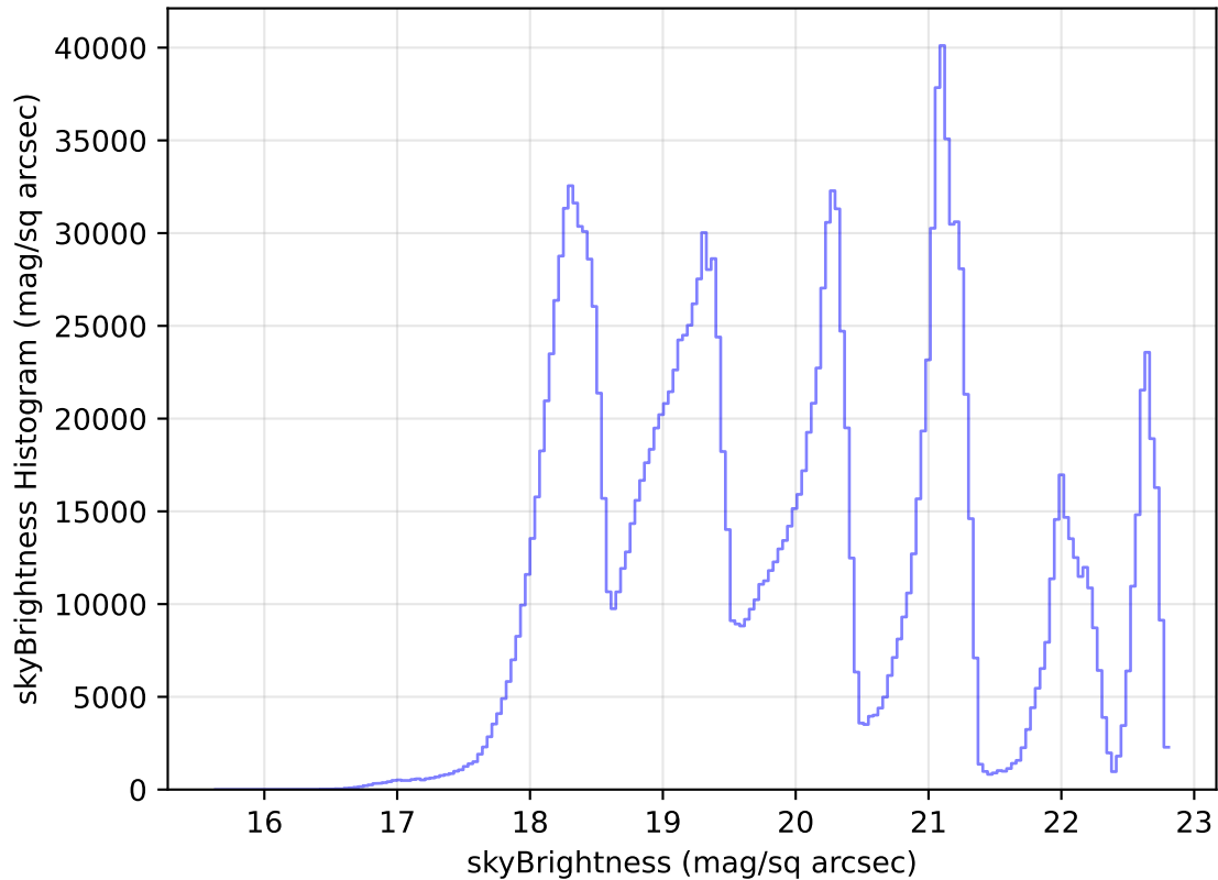
internal_u_expt30_nscale1.1v3.4_10yrs All sky all bands: skyBrightness Histogram
