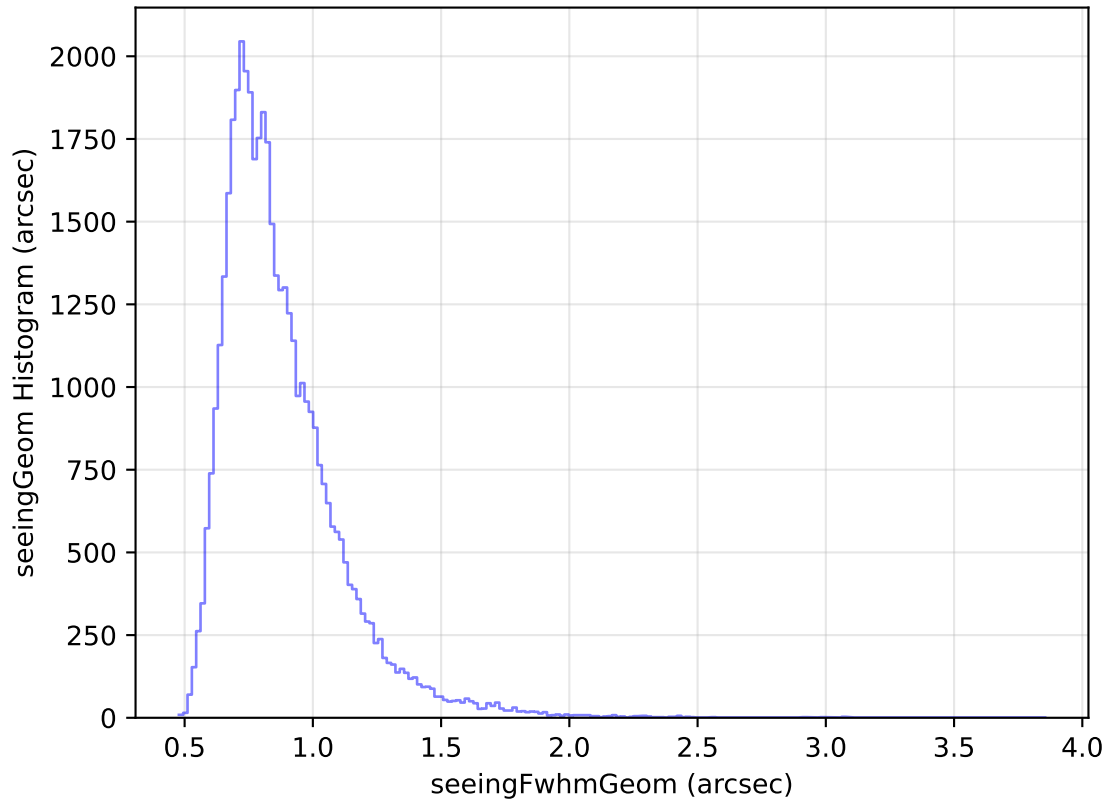
internal_u_expt30_nscale1.1v3.4_10yrs Yr 1 z band: seeingGeom Histogram
