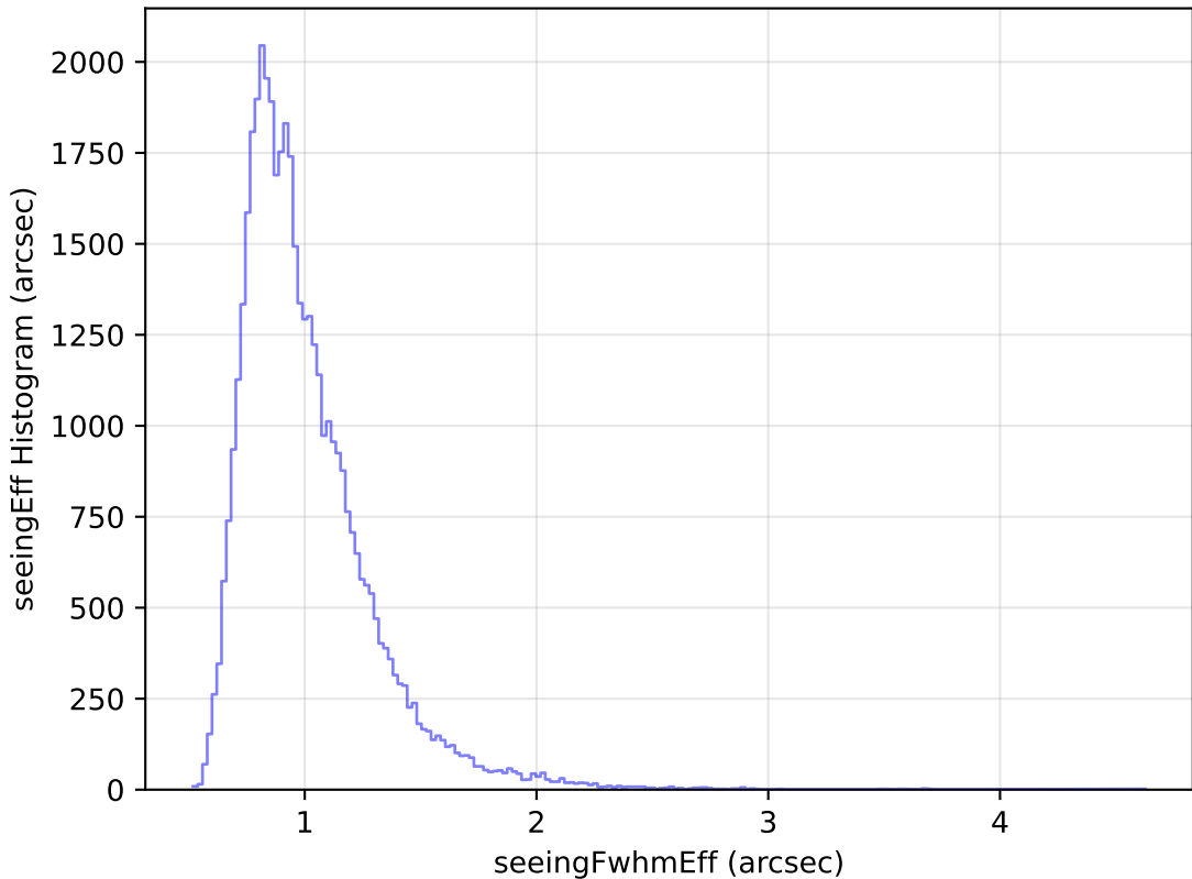
internal_u_expt30_nscale1.1v3.4_10yrs Yr 1 z band: seeingEff Histogram
