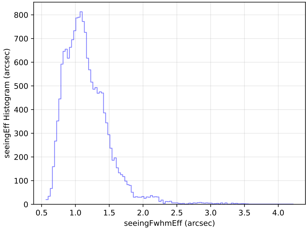
internal_u_expt30_nscale1.1v3.4_10yrs Yr 1 u band: seeingEff Histogram
