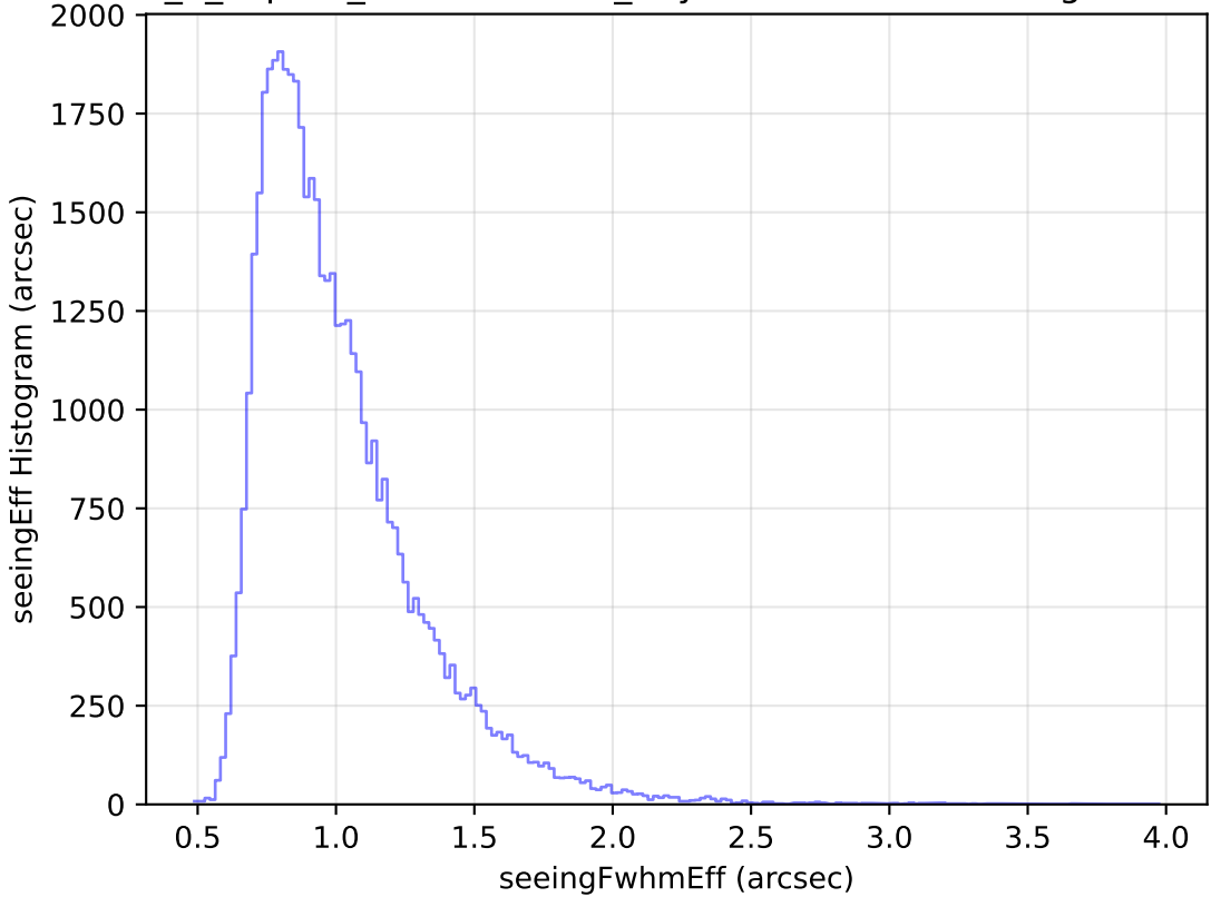
internal_u_expt30_nscale1.1v3.4_10yrs Yr 1 r band: seeingEff Histogram
