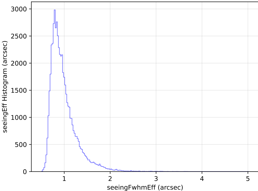
internal_u_expt30_nscale1.1v3.4_10yrs Yr 1 i band: seeingEff Histogram
