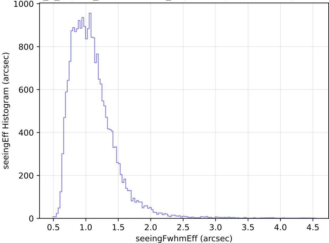
internal_u_expt30_nscale1.1v3.4_10yrs Yr 1 g band: seeingEff Histogram
