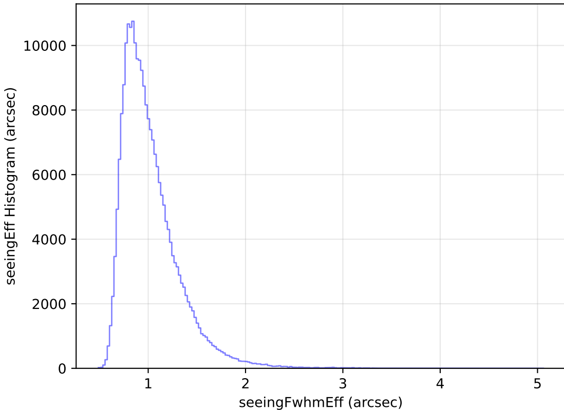
internal_u_expt30_nscale1.1v3.4_10yrs Yr 1 all bands: seeingEff Histogram
