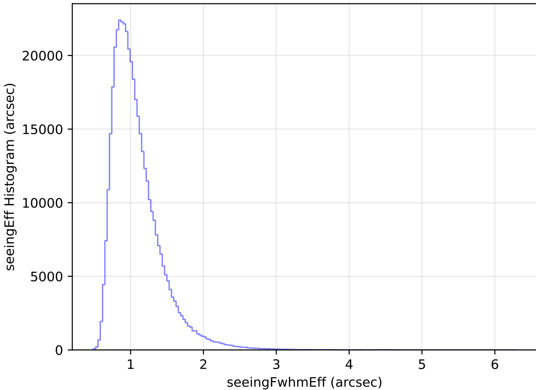
internal_u_expt30_nscale1.1v3.4_10yrs WFD z band: seeingEff Histogram
