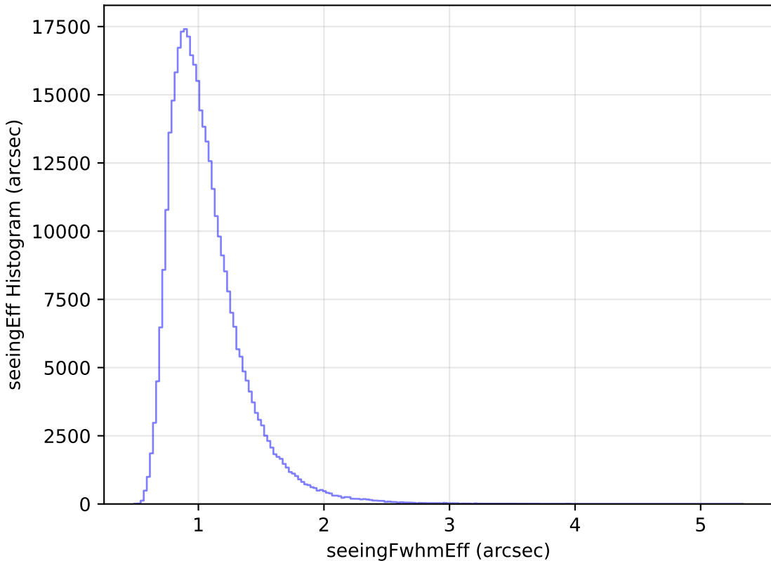
internal_u_expt30_nscale1.1v3.4_10yrs WFD y band: seeingEff Histogram
