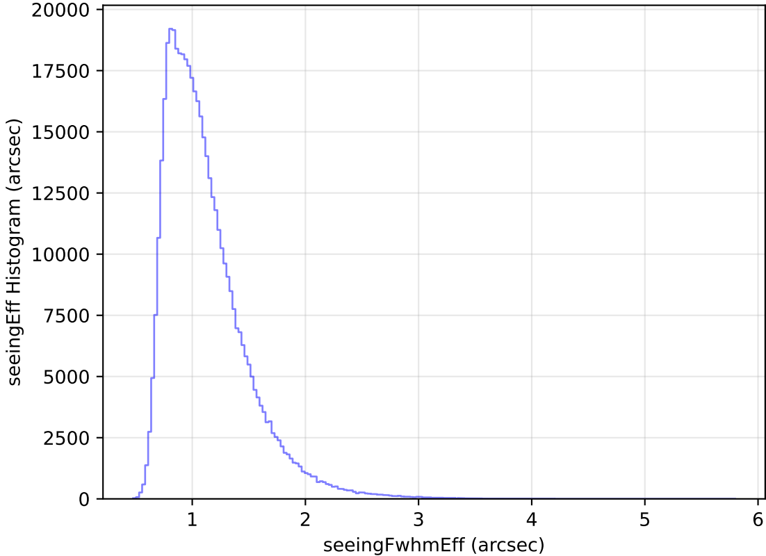
internal_u_expt30_nscale1.1v3.4_10yrs WFD r band: seeingEff Histogram
