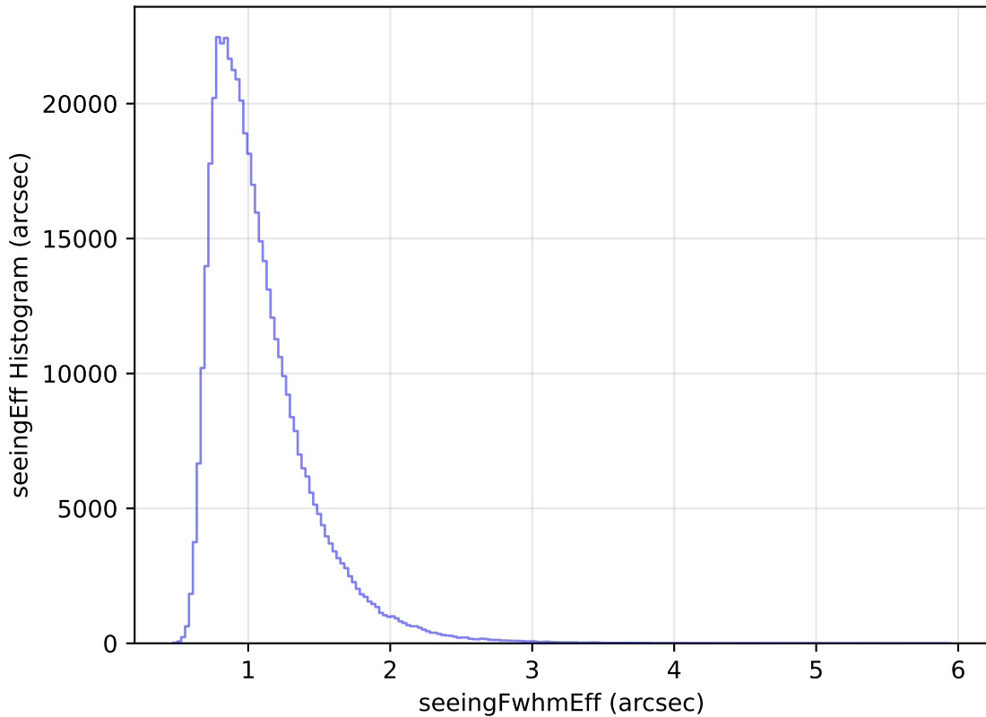
internal_u_expt30_nscale1.1v3.4_10yrs WFD i band: seeingEff Histogram
