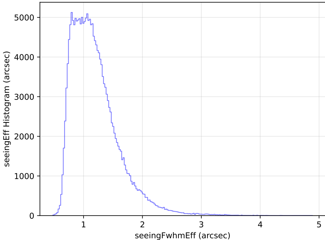
internal_u_expt30_nscale1.1v3.4_10yrs WFD g band: seeingEff Histogram
