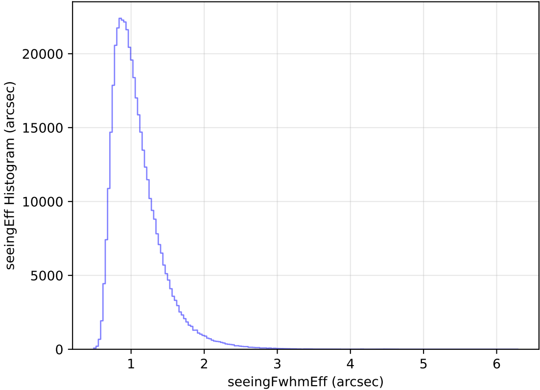
internal_u_expt30_nscale1.1v3.4_10yrs All sky z band: seeingEff Histogram
