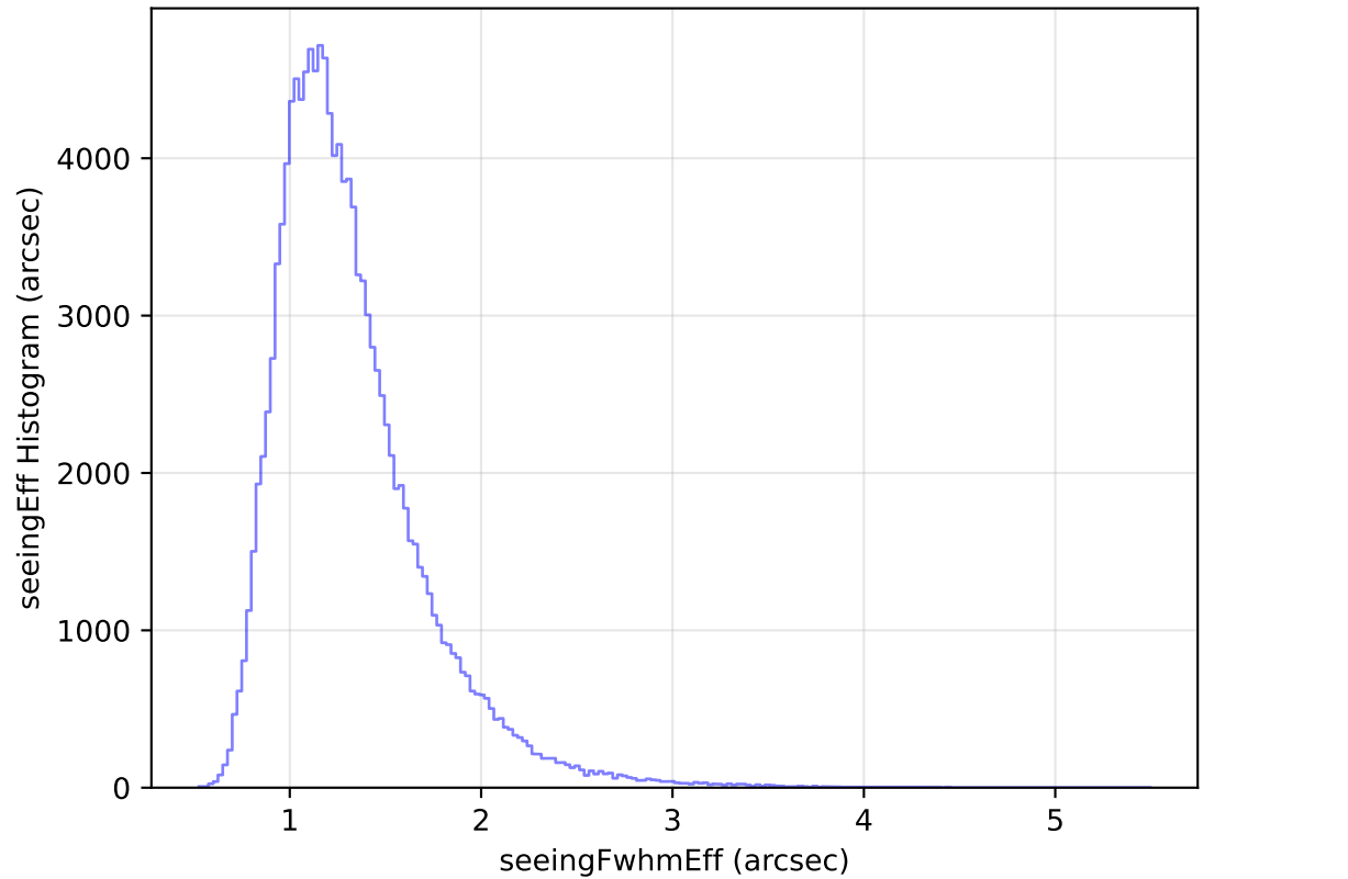
internal_u_expt30_nscale1.1v3.4_10yrs All sky u band: seeingEff Histogram
