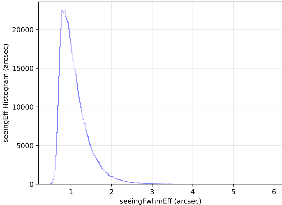
internal_u_expt30_nscale1.1v3.4_10yrs All sky i band: seeingEff Histogram
