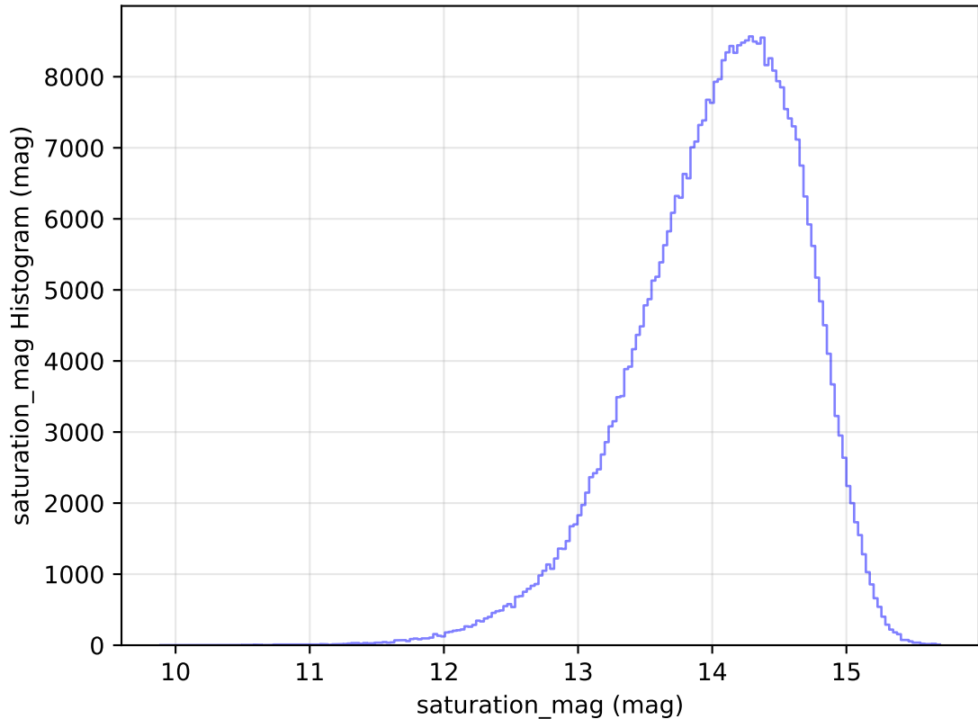
internal_u_expt30_nscale1.1v3.4_10yrs WFD z band: saturation_mag Histogram
