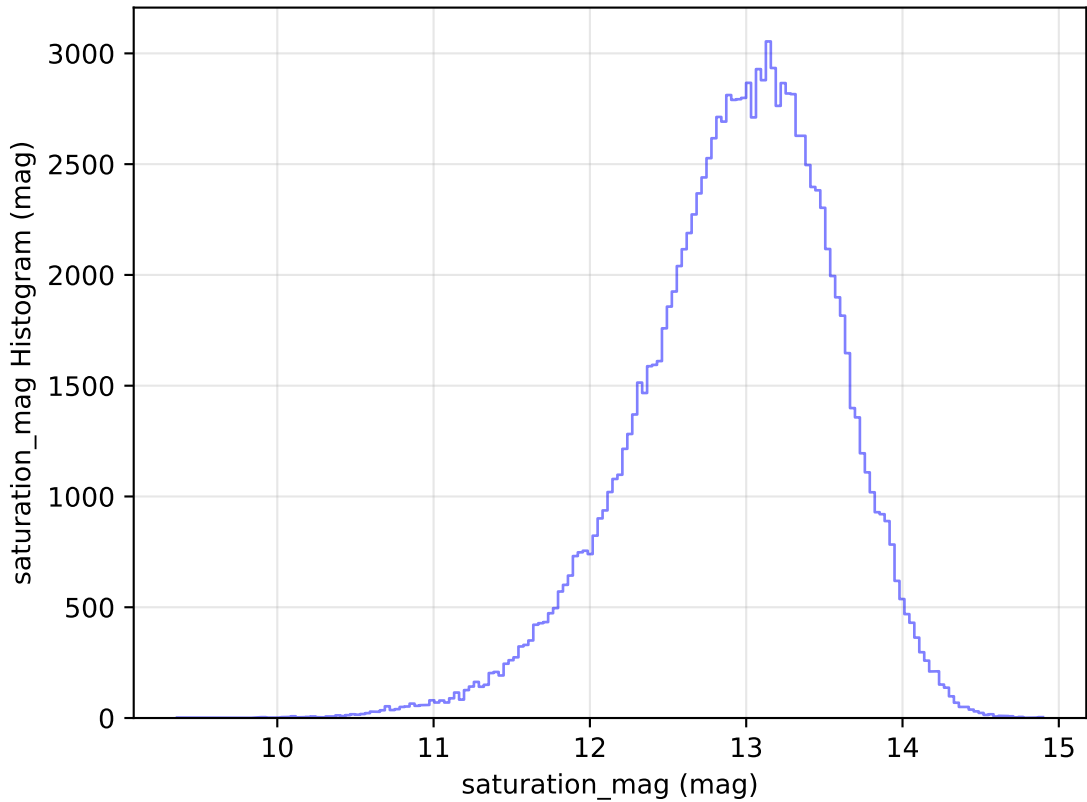
internal_u_expt30_nscale1.1v3.4_10yrs WFD u band: saturation_mag Histogram
