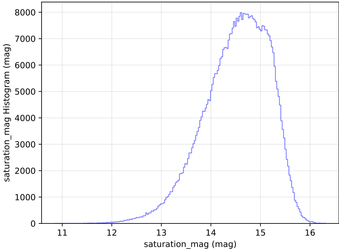
internal_u_expt30_nscale1.1v3.4_10yrs WFD r band: saturation_mag Histogram
