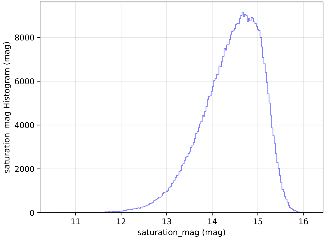
internal_u_expt30_nscale1.1v3.4_10yrs WFD i band: saturation_mag Histogram
