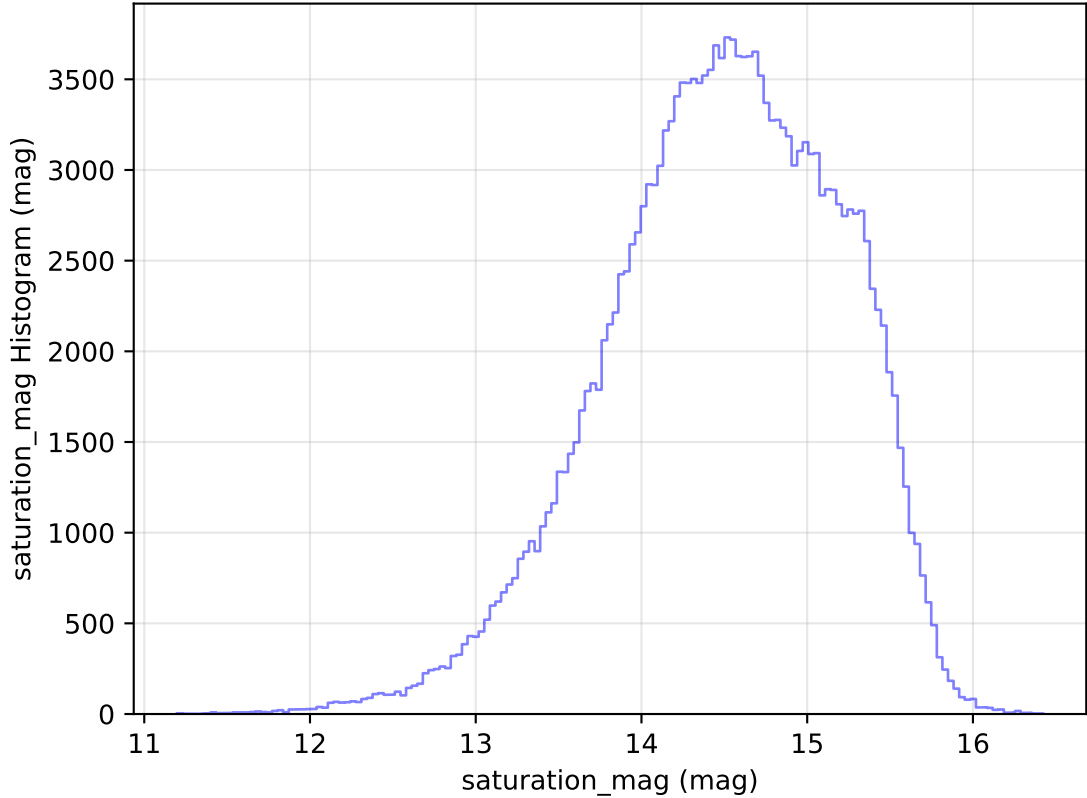
internal_u_expt30_nscale1.1v3.4_10yrs WFD g band: saturation_mag Histogram
