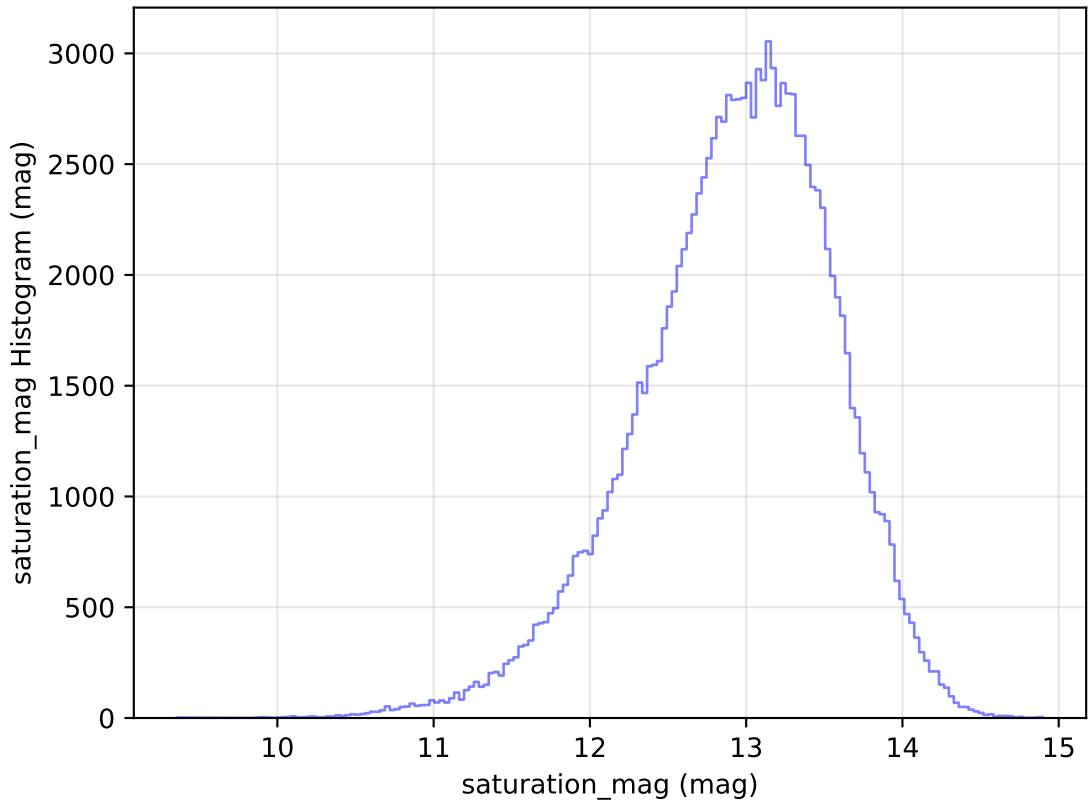
internal_u_expt30_nscale1.1v3.4_10yrs All sky u band: saturation_mag Histogram
